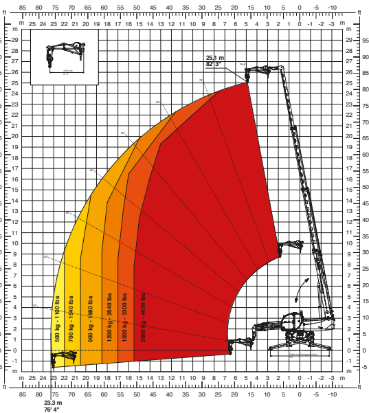
REP 2-4,5 Rotating extendable men platform 1100 lbs
