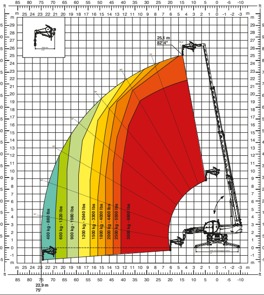
REP 10.2-4,7 Rotating extendable men platform 2200 lb
