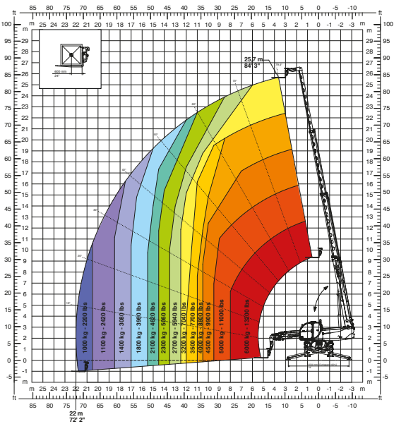
H 6 13200 lbs hook
